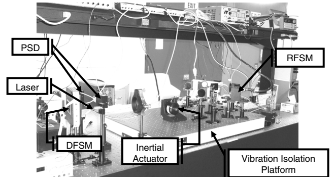
Fig. 2 Laser jitter control test bed.
