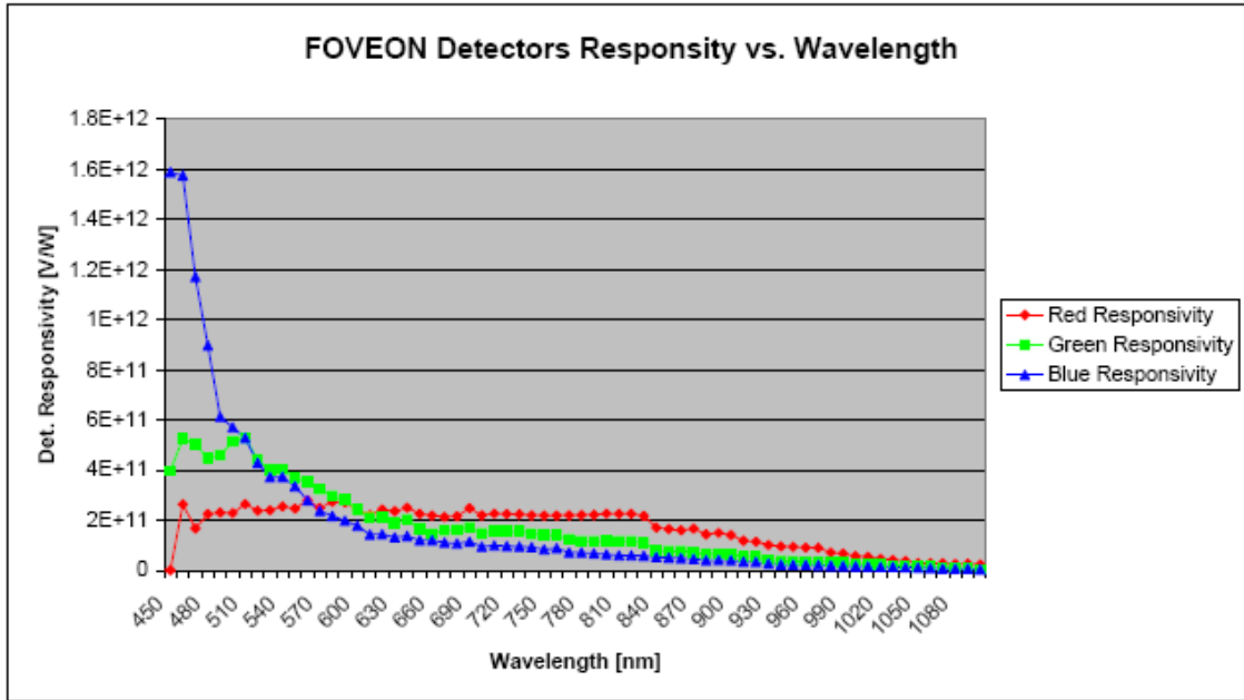
Figure 26. FOVEON Sensor Signals vs. wavelength [above], FOVEON Sensor Responsivity vs. wavelength [below]
