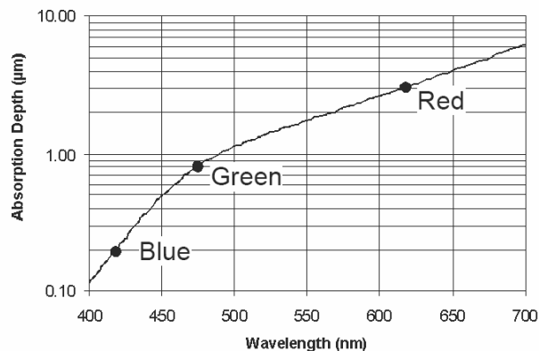
Figure 2. Absorption Depth of Silicon with Wavelength. The photodetectors used in FOVEON camera are located at the three depths of 0.2 µm, 0.8 µm and 3 µm [4].
