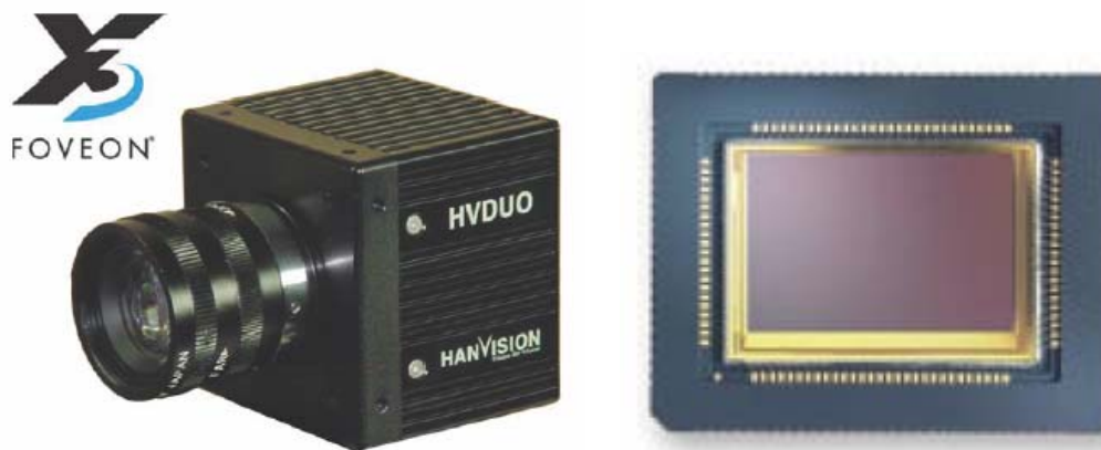
Figure 9. The HanVision HVDUO-5M Camera (left) [8] and the internal FOVEON X3 Image Sensor (right) [4].
