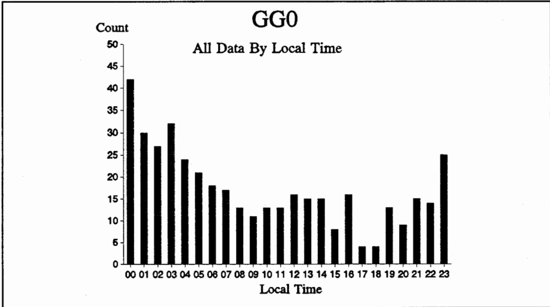
Figure 27. Local time distribution of all GG0 anomalies.
