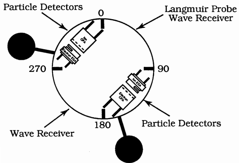
Figure 3. Particle Detector Orientations
