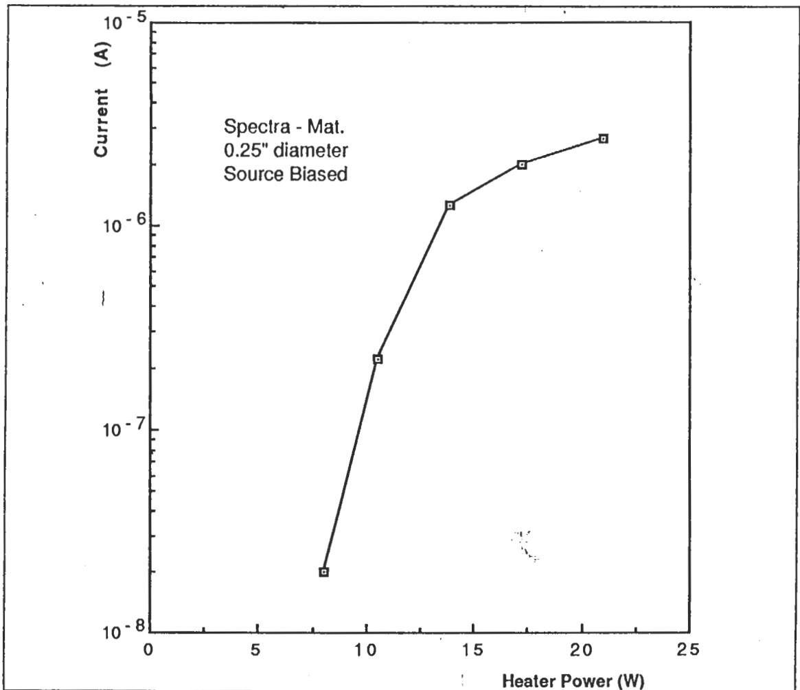
Figure 28. Emission current versus applied power: ground the mesh, bias to source + 100 V w.r.t. mesh, bias + 10 V w.r.t. metal strips.
