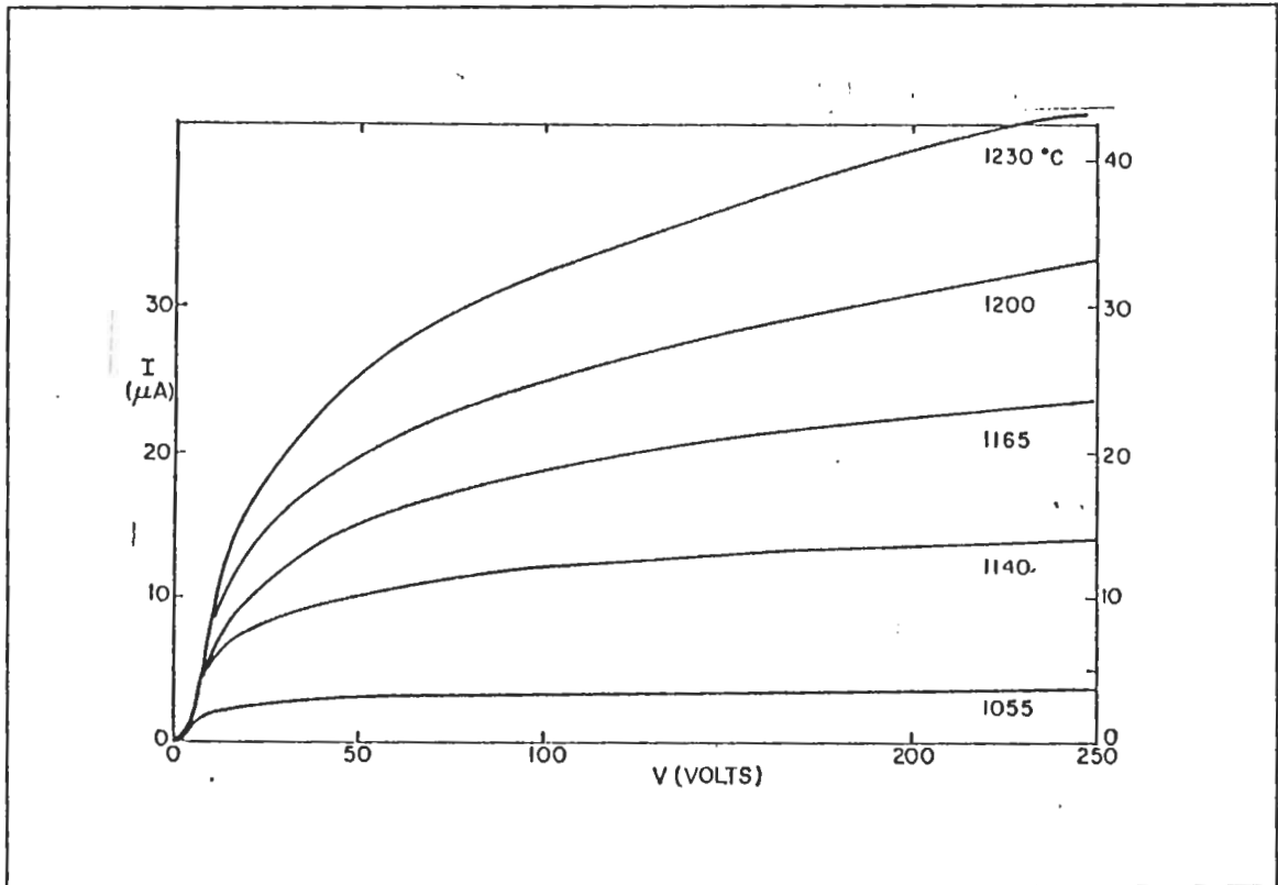
Figure 7. Typical diode characteristics of current vs voltage. [Ref.6]
