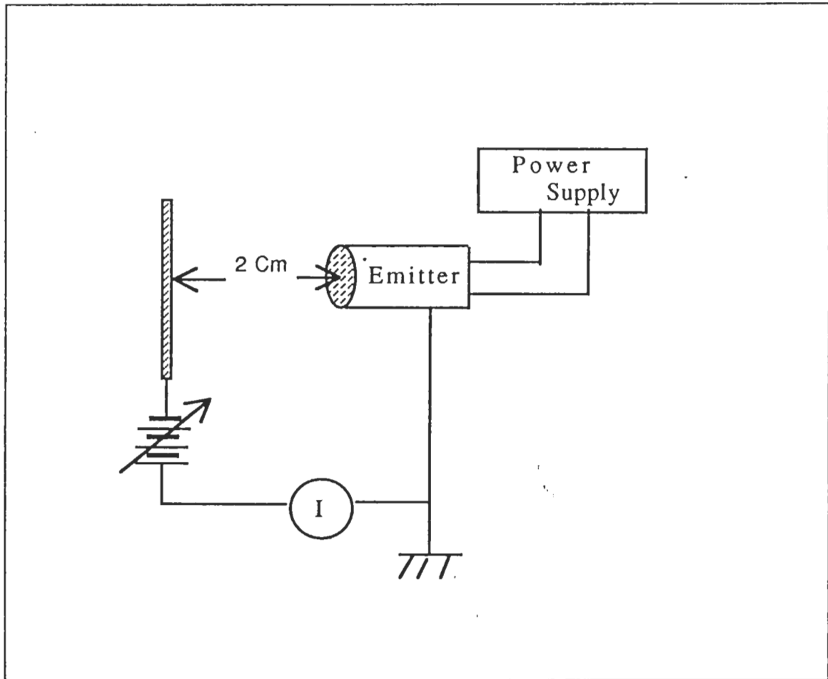
Figure 18. Diagram for measuring total current
