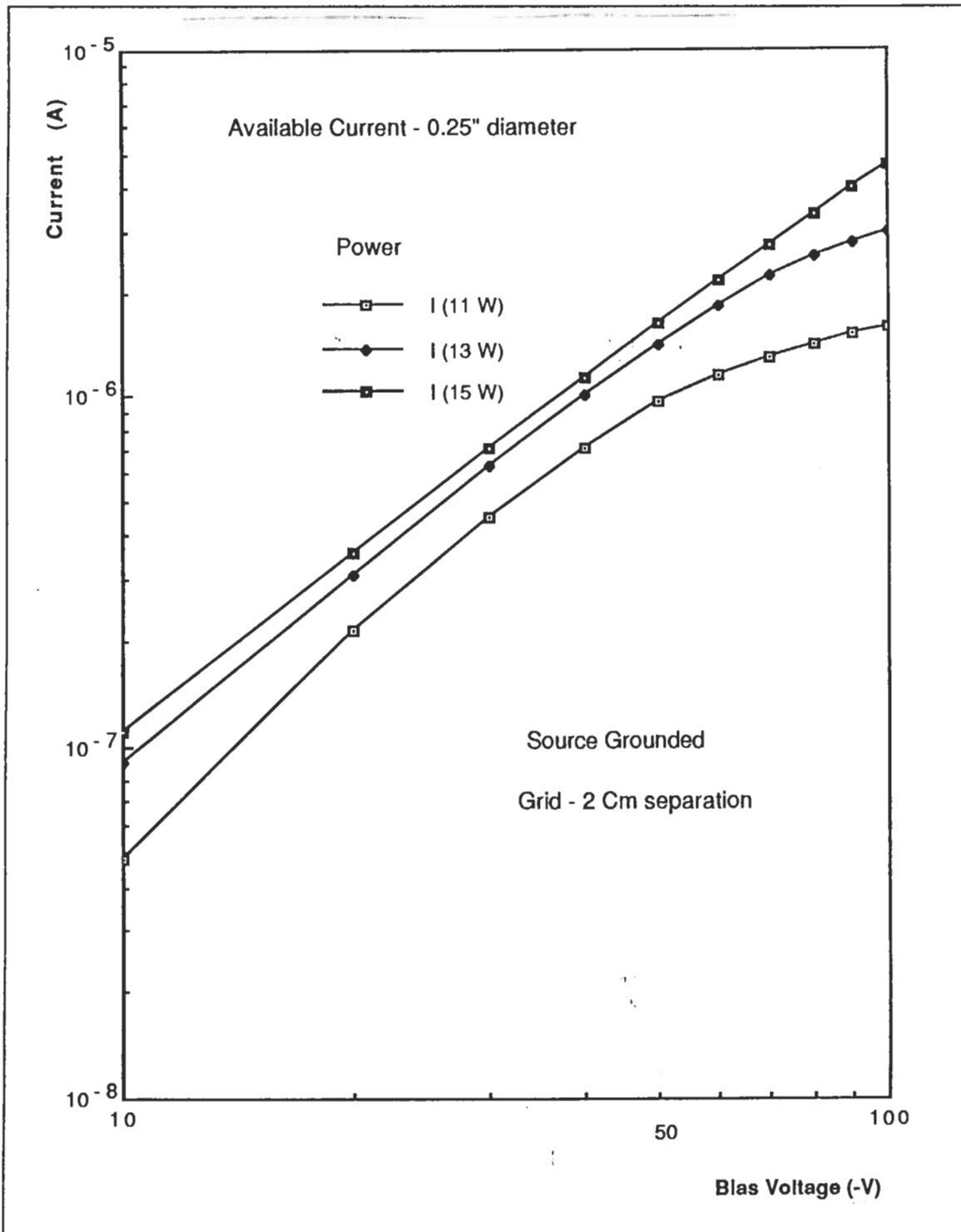
Figure 19. Emitting current as function of bias voltage to grid (negative).
