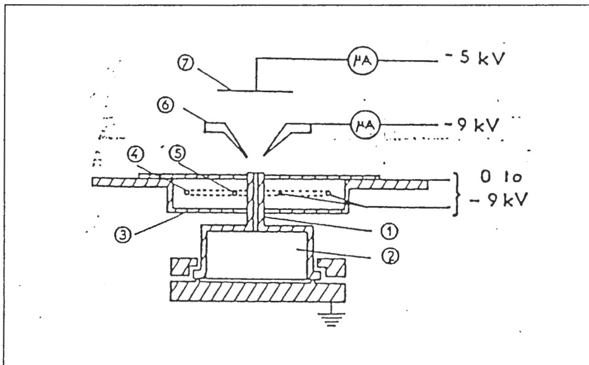
Figure 11. Cross section of the lithium capillary ion source: (1)Capillary tube, (2)lithium reservoir, (3)electron reflector, (4)Hot tungsten filament, (5)cold filament, (6)extractor, (7)collector. [Ref.11]
