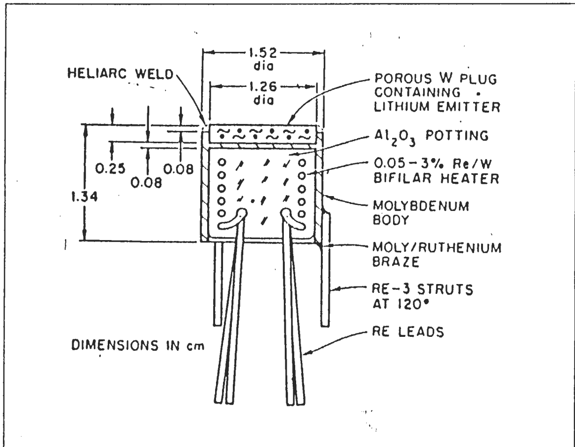
Figure 9. Construction of Lithium Ion Emitter. [Ref.2]
