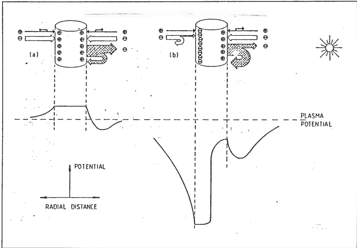
Figure 2. Schematic representation of particle flows.: (a)a conductive surface (b) an insulator surface. [Ref.1]
