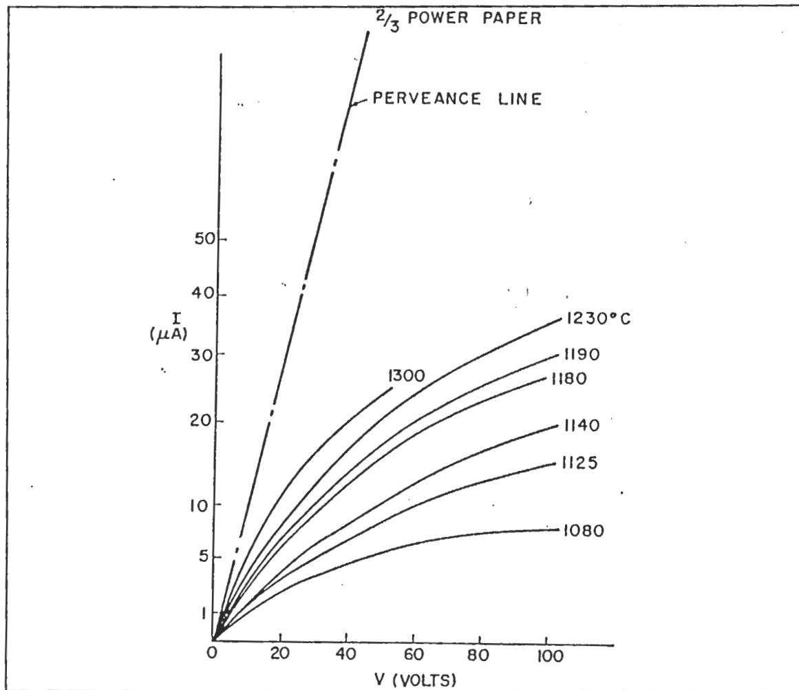
Figure 8. Typical plot of I^{2/3} versus V for a lithium ion emitter.: The perveance line applies to the Child-Langmuir equation. [Ref.6]
