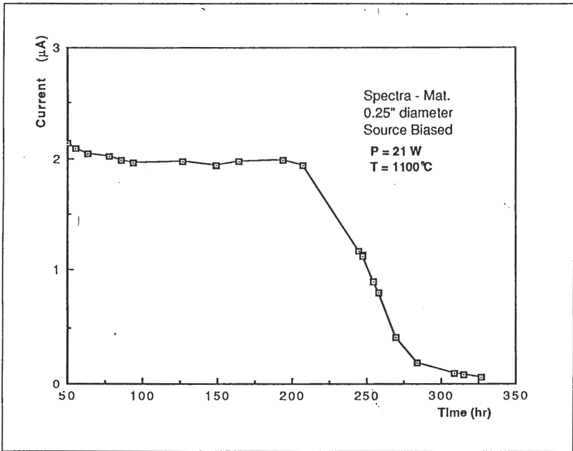
Figure 31. Emission current as function of operating Time.
