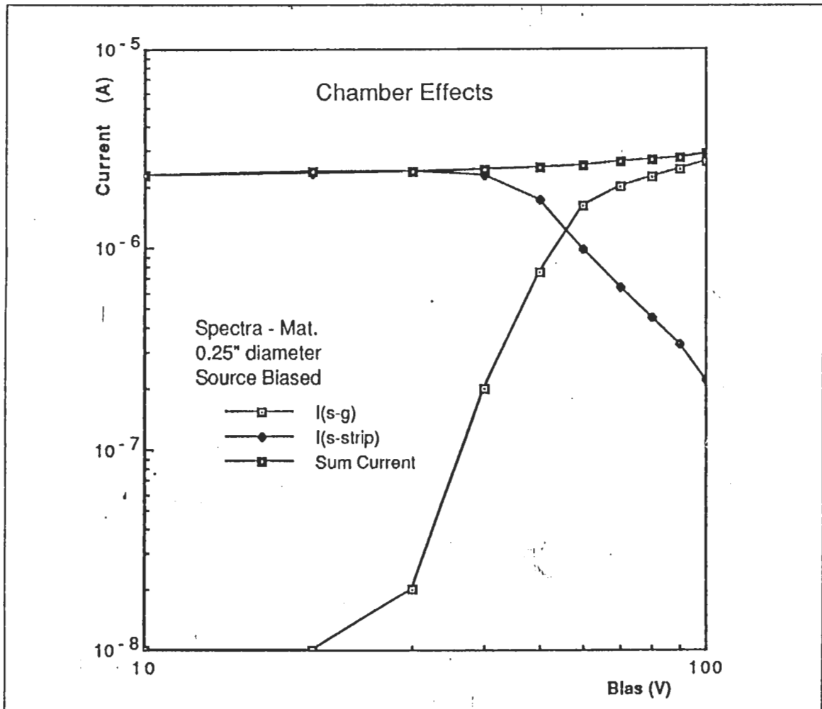
Figure 29. Emission current versus bias voltage to source w.r.t. mesh: ground the mesh, bias to source + 10 V w.r.t. metal strips, power 21 W.
