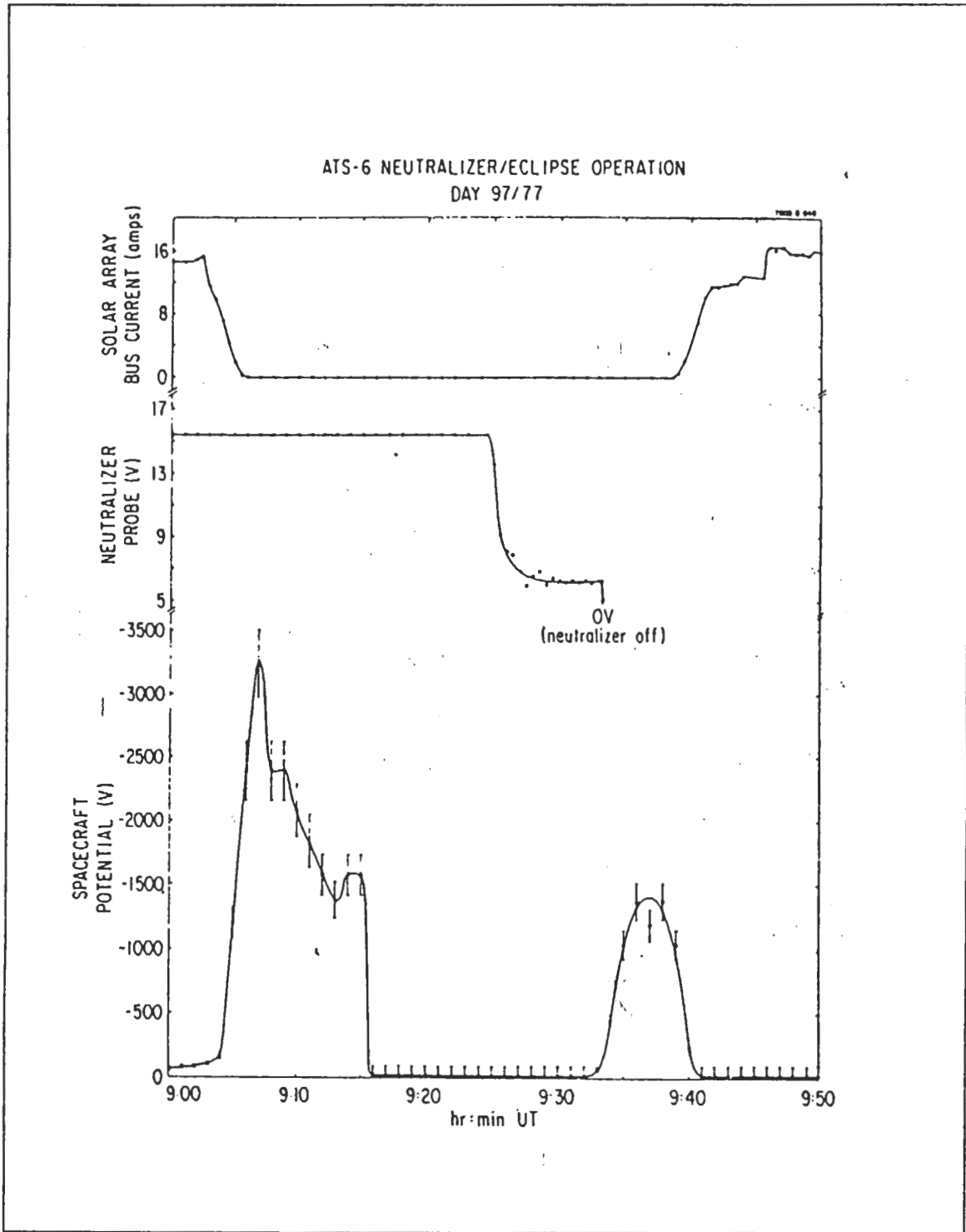
Figure 5. Plasma bridge operation, April 7, 1977 [Ref.5]
