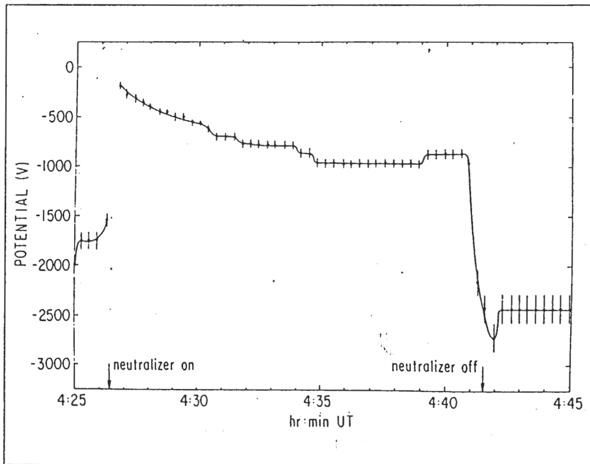
Figure 4. ATS-5 neutralizer operation, March 28, 1978 [Ref.4]
