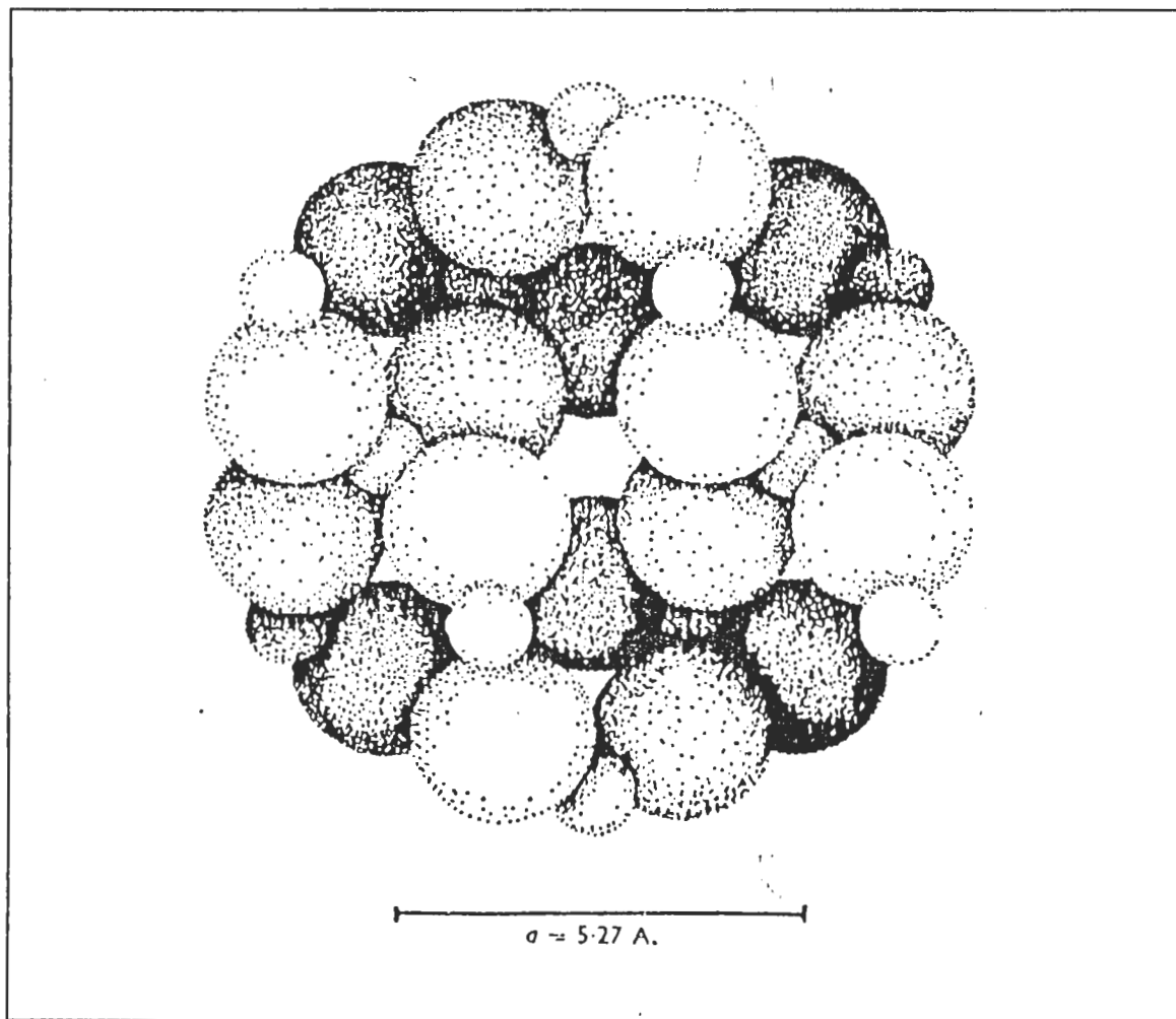
Figure 6. Crystal structure of \beta -eucryptite viewed along c axis.: Large spheres represents oxygen atoms, small spheres either Si or Al atoms. The lithium ions are situated in center opening. [Ref.6]
