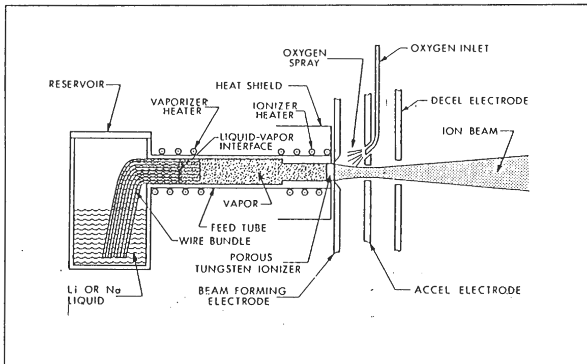
Figure 13. Schematic representation of the ion source configuration: used to generate lithium and sodium ions. [Ref.12]
