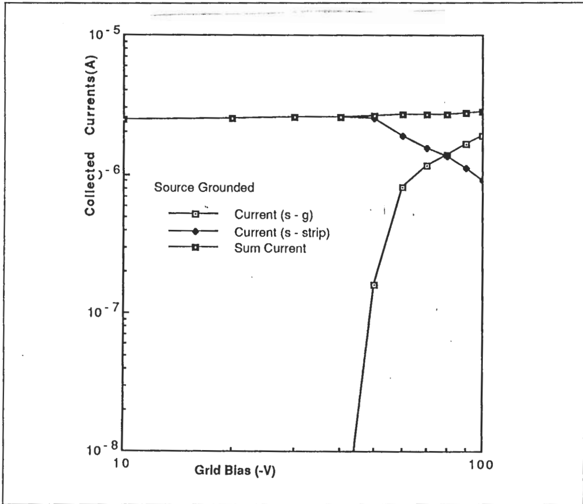
Figure 25. Emission current as function of bias voltage to mesh: w.r.t. source, at power 21 W, Temp. 1148°C, bias -10 V to strips.
