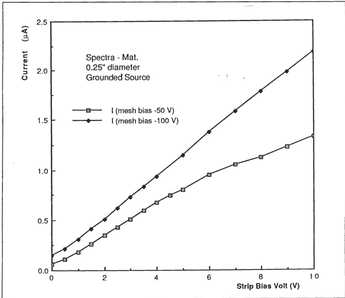
Figure 24. Emission current as function of bias voltage negative: to metal strips with respect to source.
