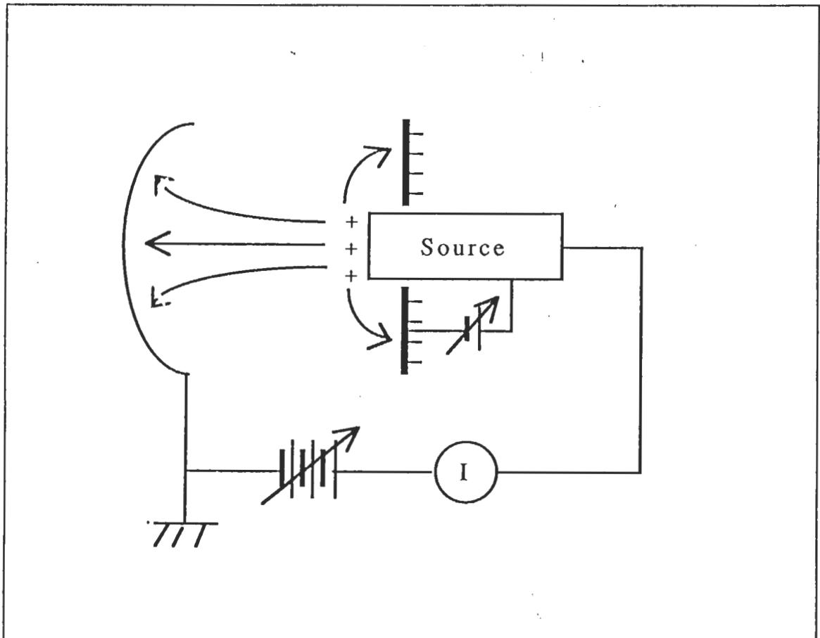
Figure 26. Diagram for checking the effect due to the geometry of chamber.
