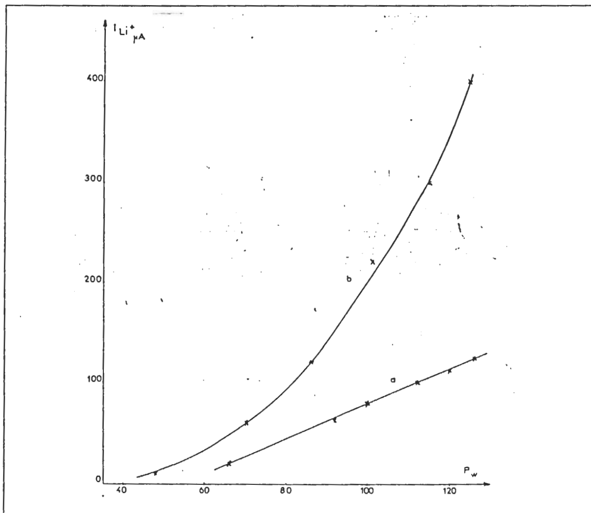
Figure 12. \text{Li}^+ ion current vs heating power.: (a)without a heat reflector (b)with a heat reflector [Ref.11]
