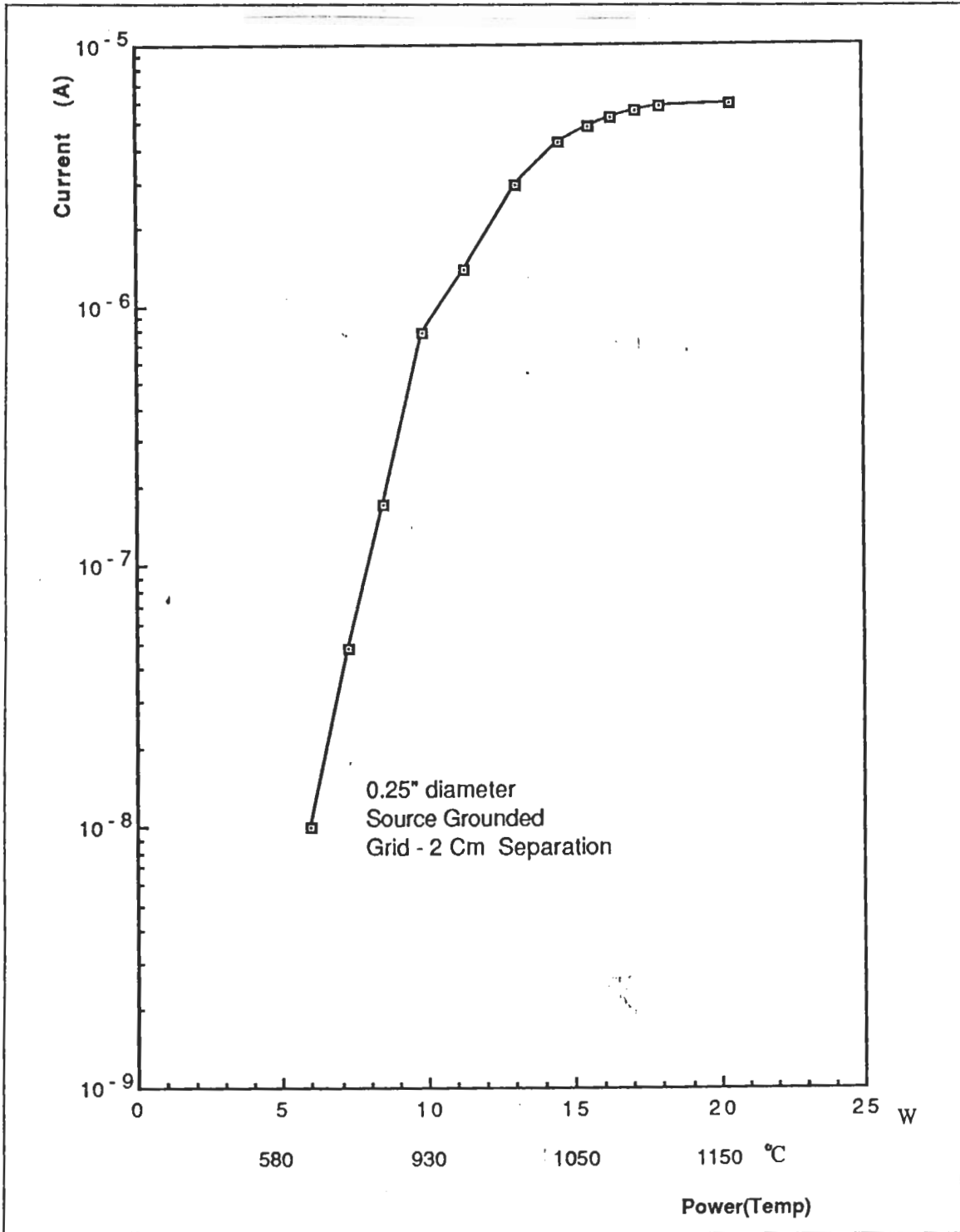
Figure 20. Total emission current as function of power (Temperature).
