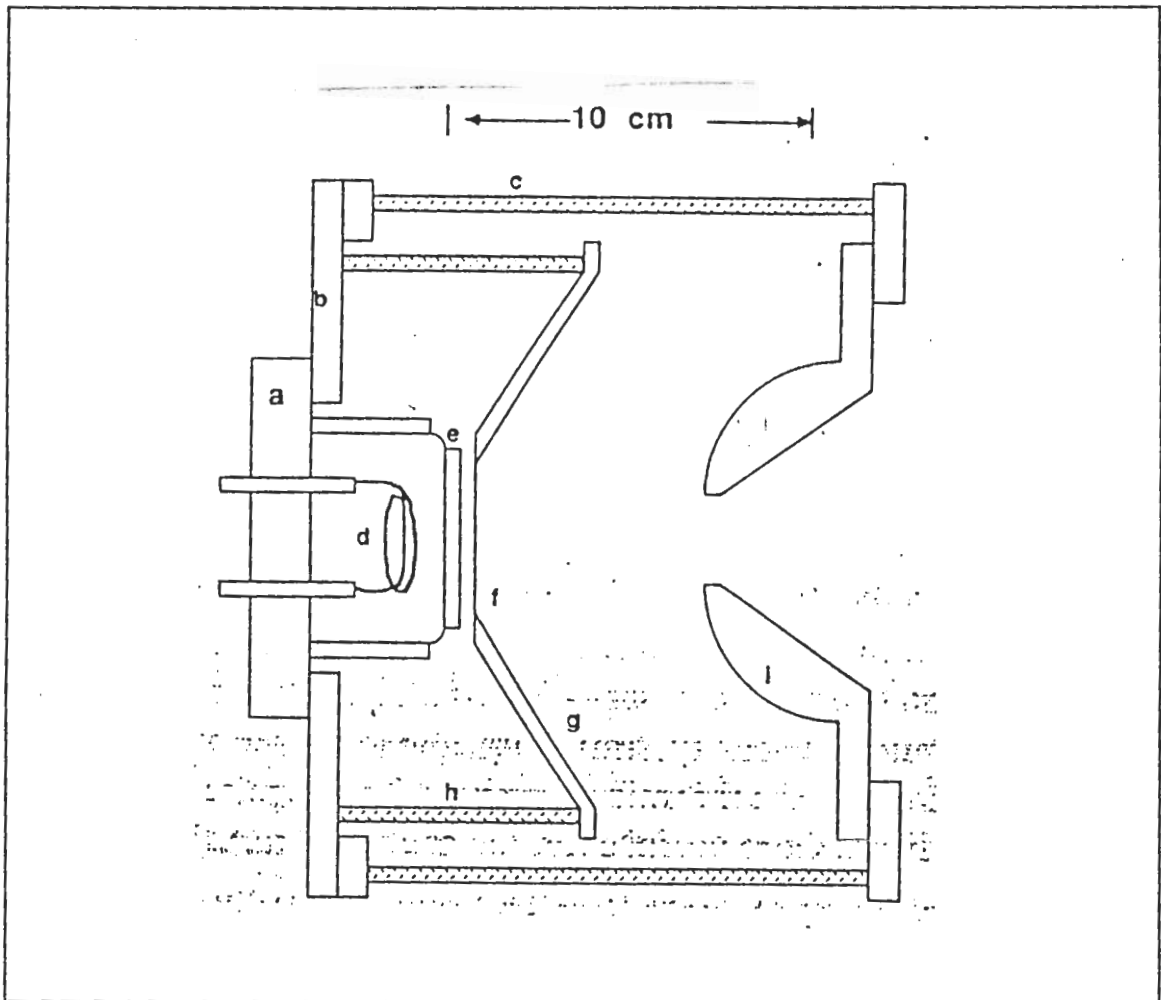
Figure 15. Sketch of the prototype lithium ion source: (a)source flange (b)gun flange (c)alumina insulator (d)heater filament (e)2-in. molybdenum disk with emissive coating (f)tungsten grid (g)cathode (h)cathode insulating support (i)anode. [Ref.16]
