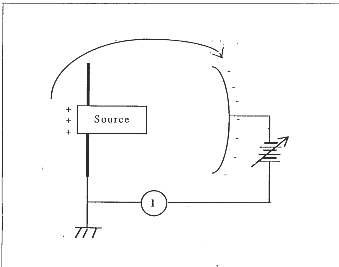
Figure 30. Diagram for control of differential charging.
