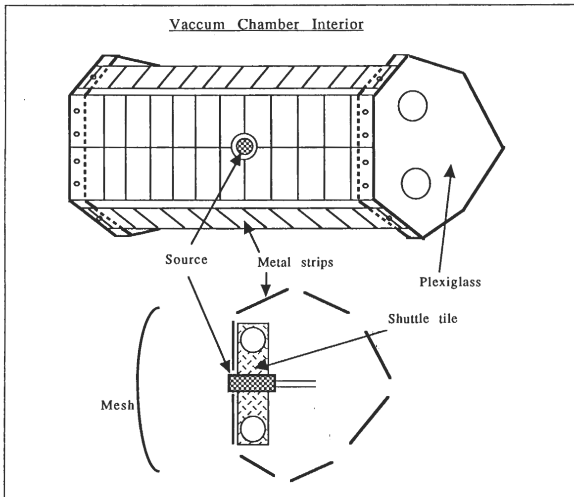
Figure 16. Vacuum chamber interior
