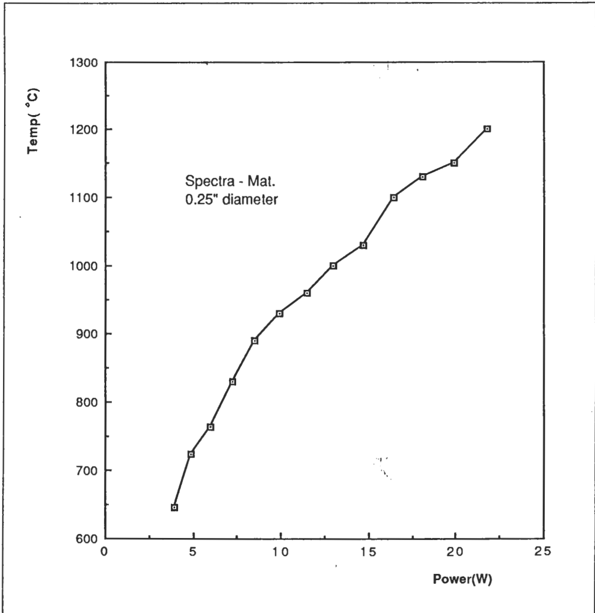
Figure 21. Source temperature as function of heater power.
