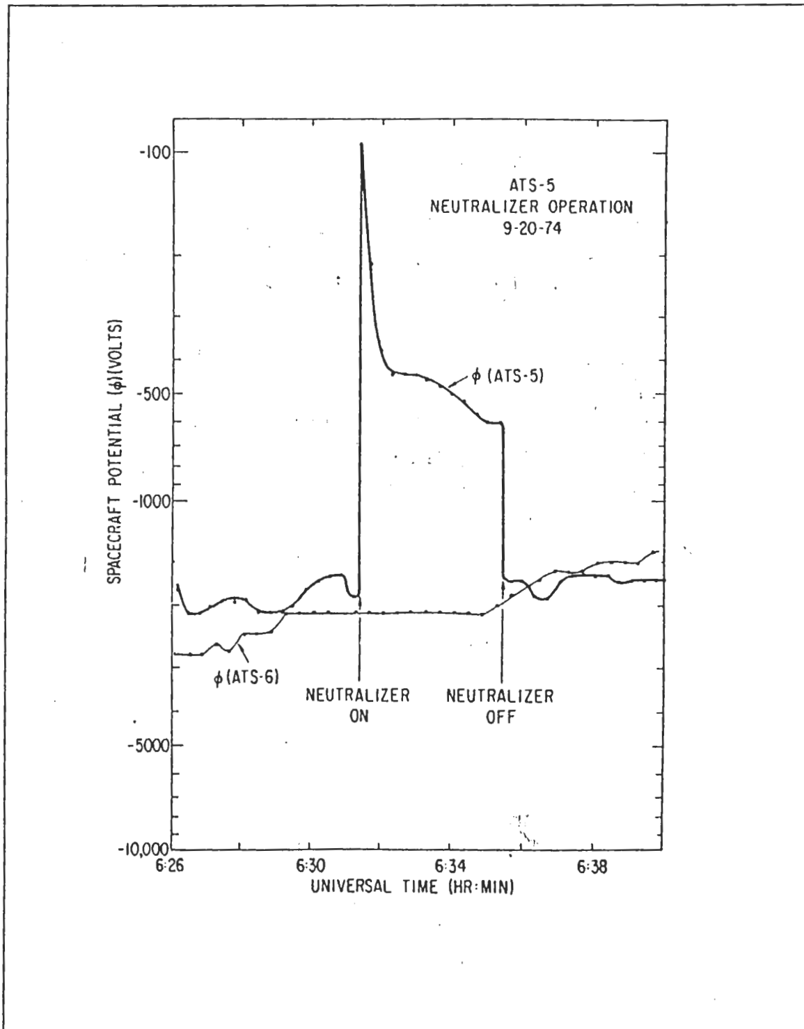
Figure 3. ATS-5 neutralizer operation, September 20, 1974[Ref.4]
