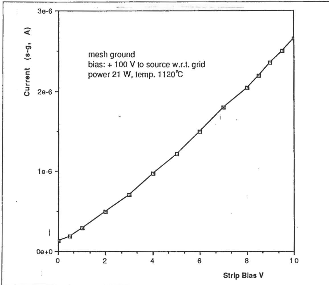
Figure 27. Emission current as function of bias voltage to strip: negative w.r.t. the source, mesh grounded.
