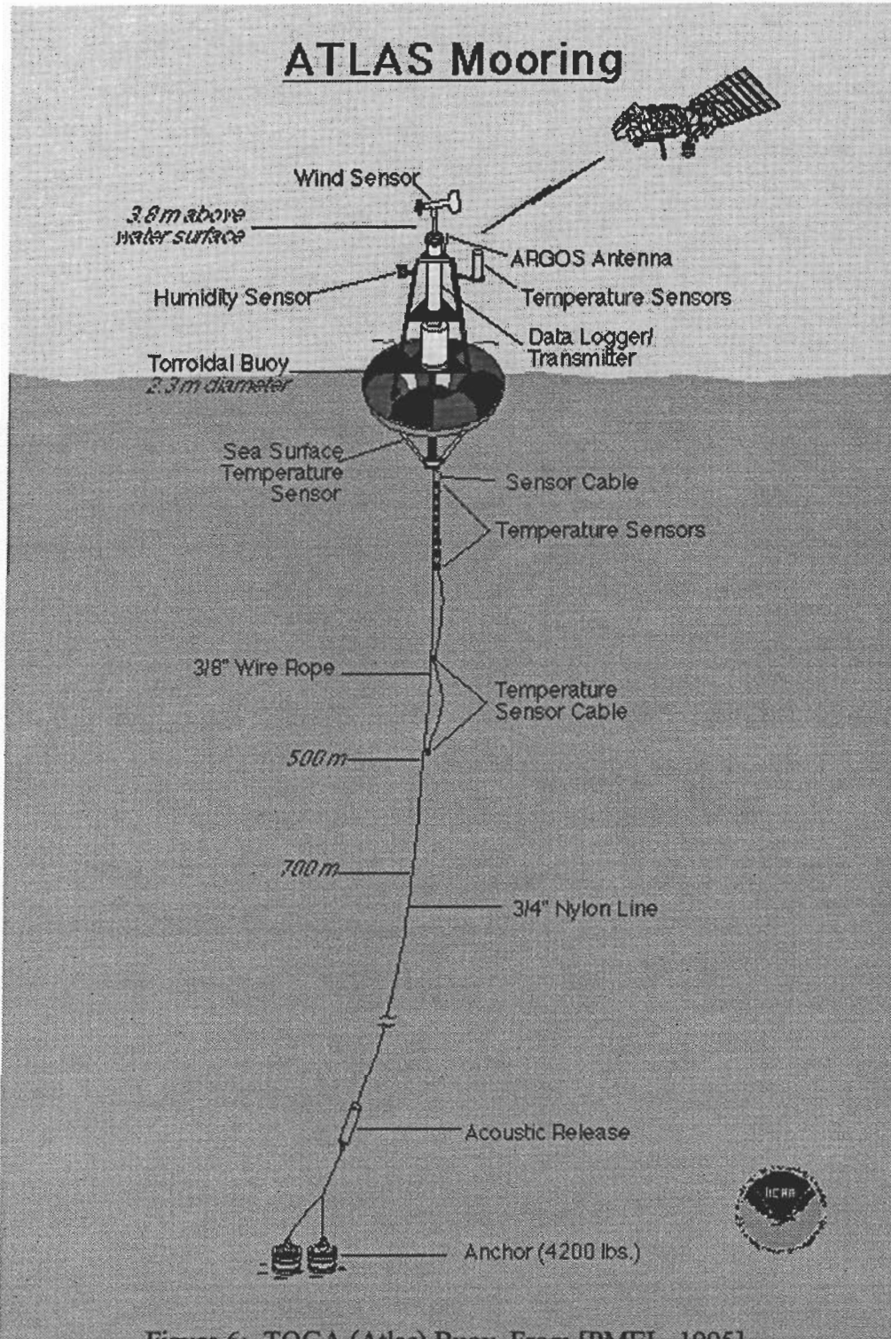
Figure 6: TOGA (Atlas) Buoy, From [PMEL, 1995]
