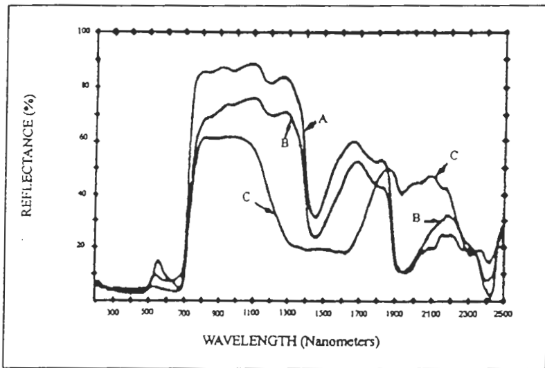
Figure 3.1 Spectral Reflectance Plot (Rinker, 1990)
