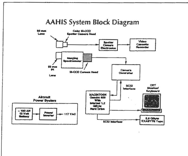
Figure 3.2 AAHIS Block Diagram
