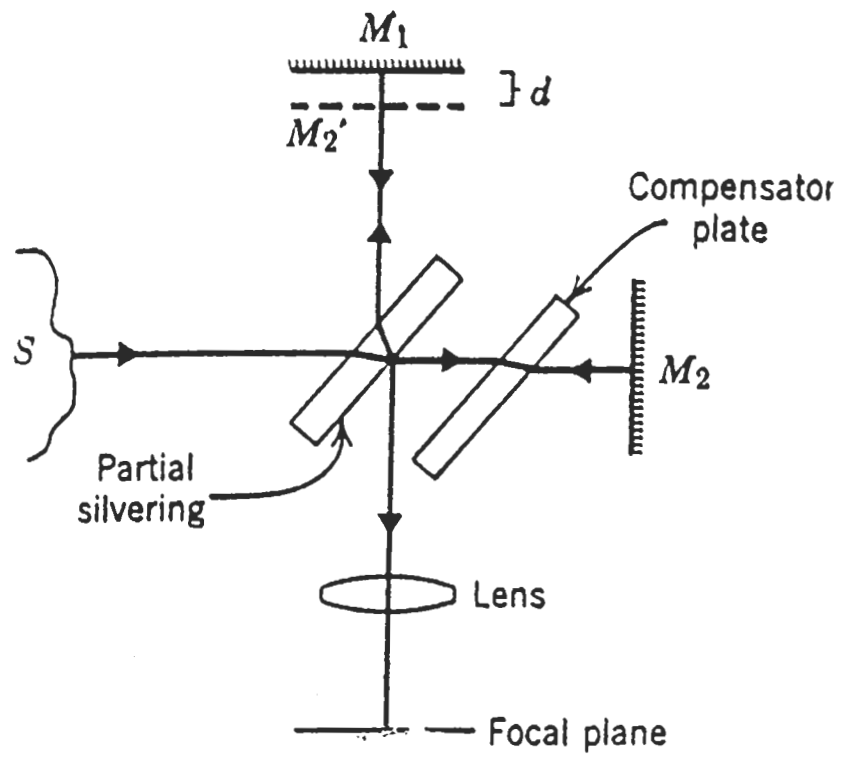
Figure 3.3 Michelson Interferometer (Klein, 1970)
