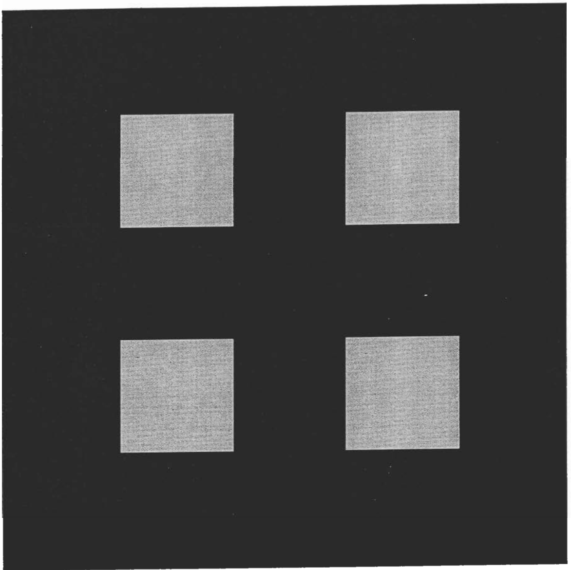
Figure 4.9 Test Image
