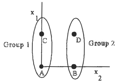
Figure 2.7 Problem definition.
