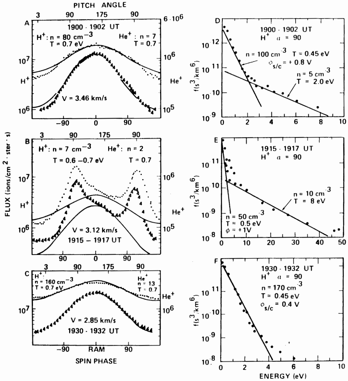
(a) Spin curves for H + (circles) and He + (4's) prior to the equator crossing, with fits. (b) Spin curves at the equator, with lines drawn for the same temperatures found in Figures 8a and 8c, at reduced densities. (c) Spin curves after the equator crossing. (d) H + distribution function for the period shown in Figure 8a. (e) H + distribution function for the period shown in Figure 8b. Note the change in energy scale as compared to Figures 8d and 8f. (f) H + distribution function for period shown in Figure 8c.
