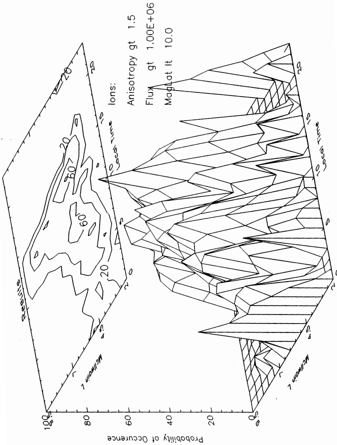
Figure 21. Trapped Ions - Flux gt 10^6 , Anisotropy gt 1.5, Maglat lt 10 - Surface Plot
