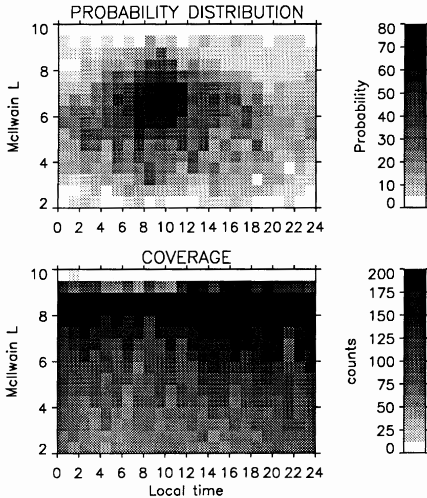
Figure 24. Trapped Electrons - Flux gt 5x10 6 , Anisotropy gt 1.5, Maglat Lt 10
