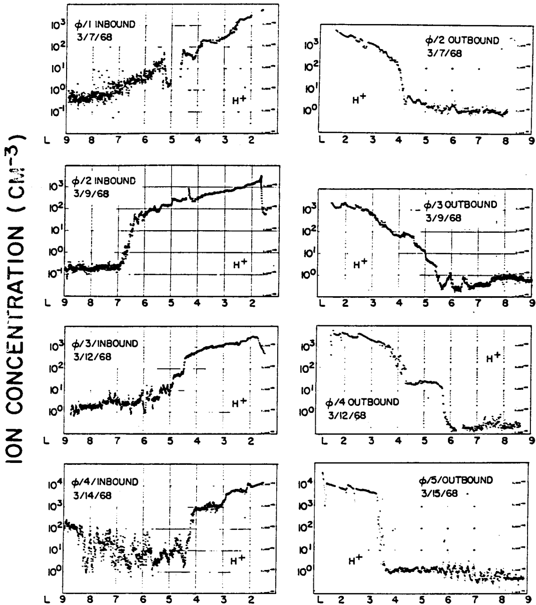
Composite of the first four H + ion concentration profiles for the inbound and outbound passes of OGO 5.
