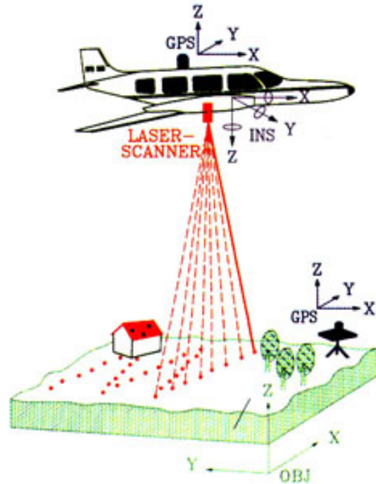
Figure 2. LIDAR Scanner Example (From: http://www.sbgmaps.com/LIDAR.htm )
