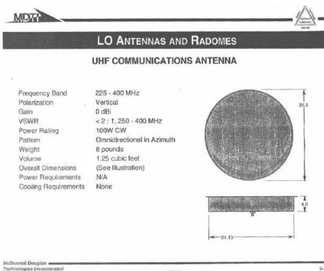
Figure IV-23. Low Observable UHF Communications Antenna
