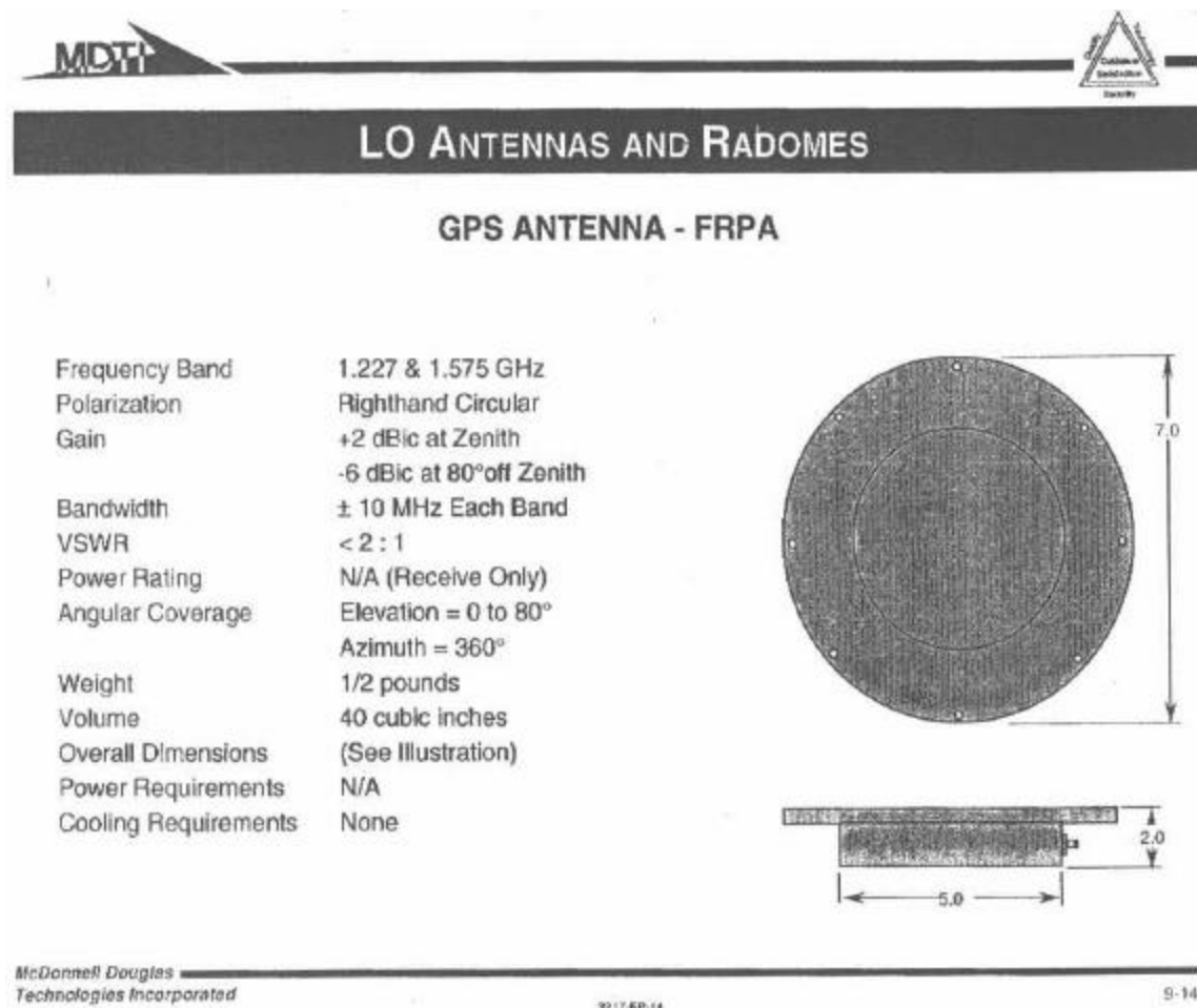
Figure IV-22. GPS antenna
