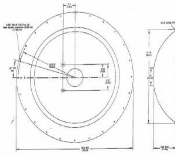
Figure IV-27. AS-3429/G
